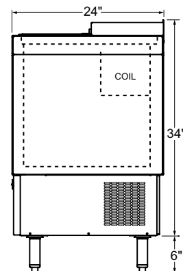
MF24 Side Elevation
