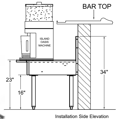
Installation Side Elevation
