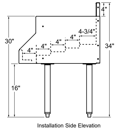
Installation Side Elevation
