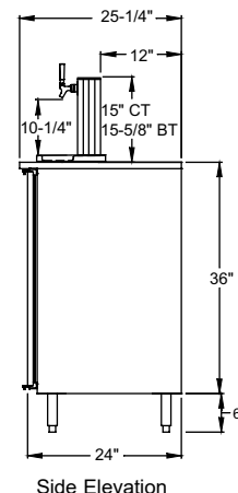
Side Elevation
