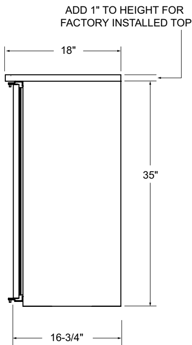
Side Elevation
