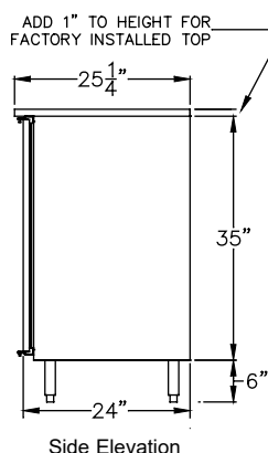
Side Elevation
